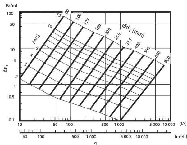
Pressure drop DZO-50
