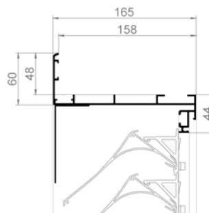
G 130HP Recessed wall louvre with flange
